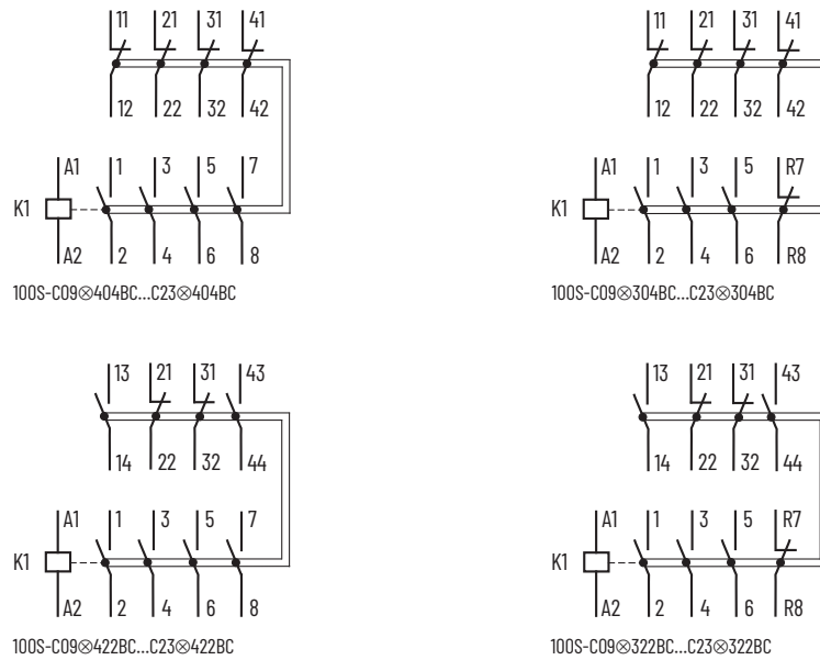
Figure 9 - Safety Contactors with 4 Main Contacts and Bifurcated Front-mount Auxiliary Contacts
