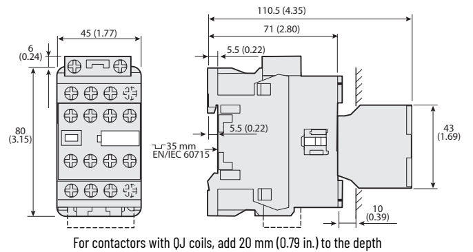
Figure 39 - 100-E09...100-E16 Contactors with Low-consumption Coils and Front-mounted Auxiliary Contact
