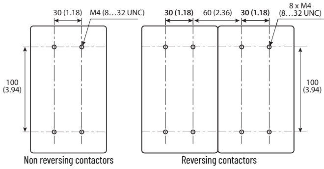
Figure 80 - 100-E190, 100-E205 Contactors
